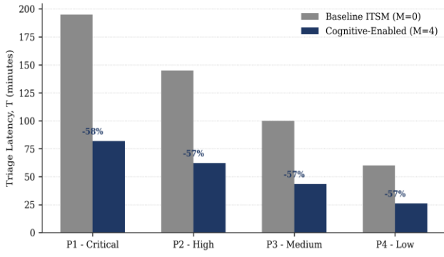
Fig. 1. Incident triage latency by severity tier (Eq. 2, M=0 vs. M=4 ).
