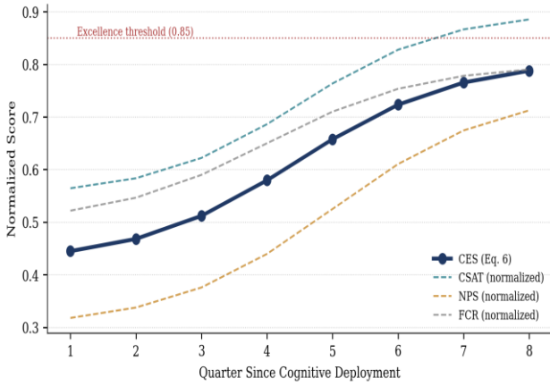
Fig. 5. Customer Experience Composite Score (CES) trend.
