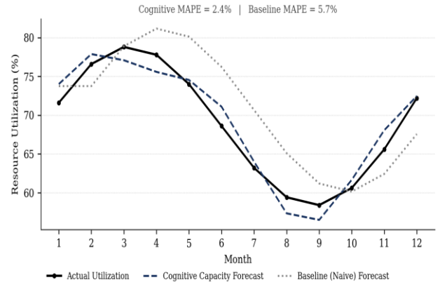
Fig. 3. Resource utilization: forecast vs. actual (12-month window).
