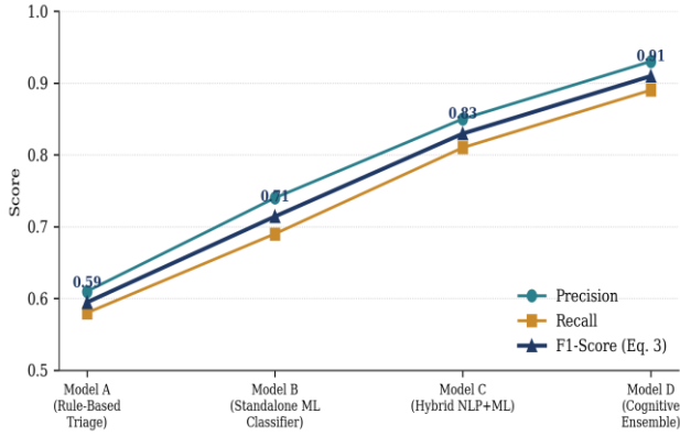
Fig. 2. Precision, recall, and F1-score across triage model architectures.
