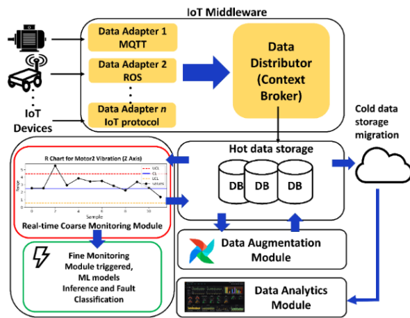
Fig 2: Architectural Frameworks
